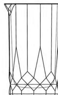
BP02810 Ø96 高156mm 容625cc MIXING B2x6/件
